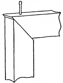
FIG. 266. METHOD OF NAILING MITER JOINT.
